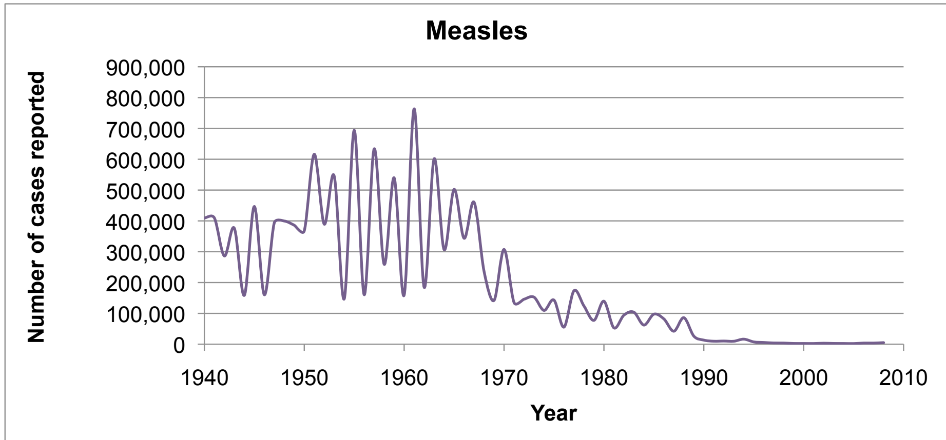
Life-saving maths: Measles Epidemics
